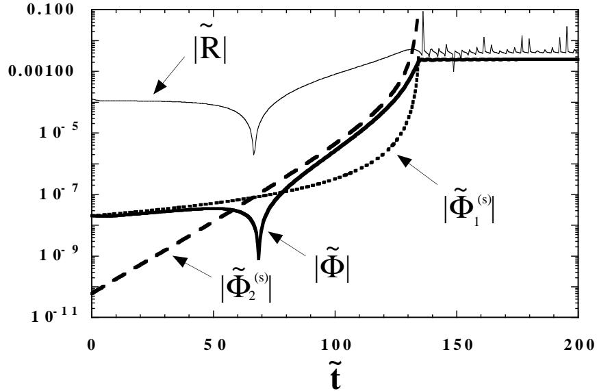
FIG. 5: The evolution of the metric perturbation \tilde{\Phi} \equiv k^{3/2}\Phi and the curvature perturbation \tilde{\mathcal{R}} \equiv k^{3/2}\mathcal{R} in the R^2 inflationary scenario with same parameters as in Fig. 4. We also plot \tilde{\Phi}_1^{(s)} \equiv k^{3/2}\Phi_1^{(s)} and \tilde{\Phi}_2^{(s)} \equiv k^{3/2}\Phi_2^{(s)} , where \Phi_1^{(s)} and \Phi_2^{(s)} denote the first and the second terms in Eq. (4.45), respectively. The evolution of \Phi_1^{(s)} and \Phi_2^{(s)} after inflation is not shown.
